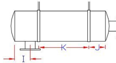
Side Inlet
